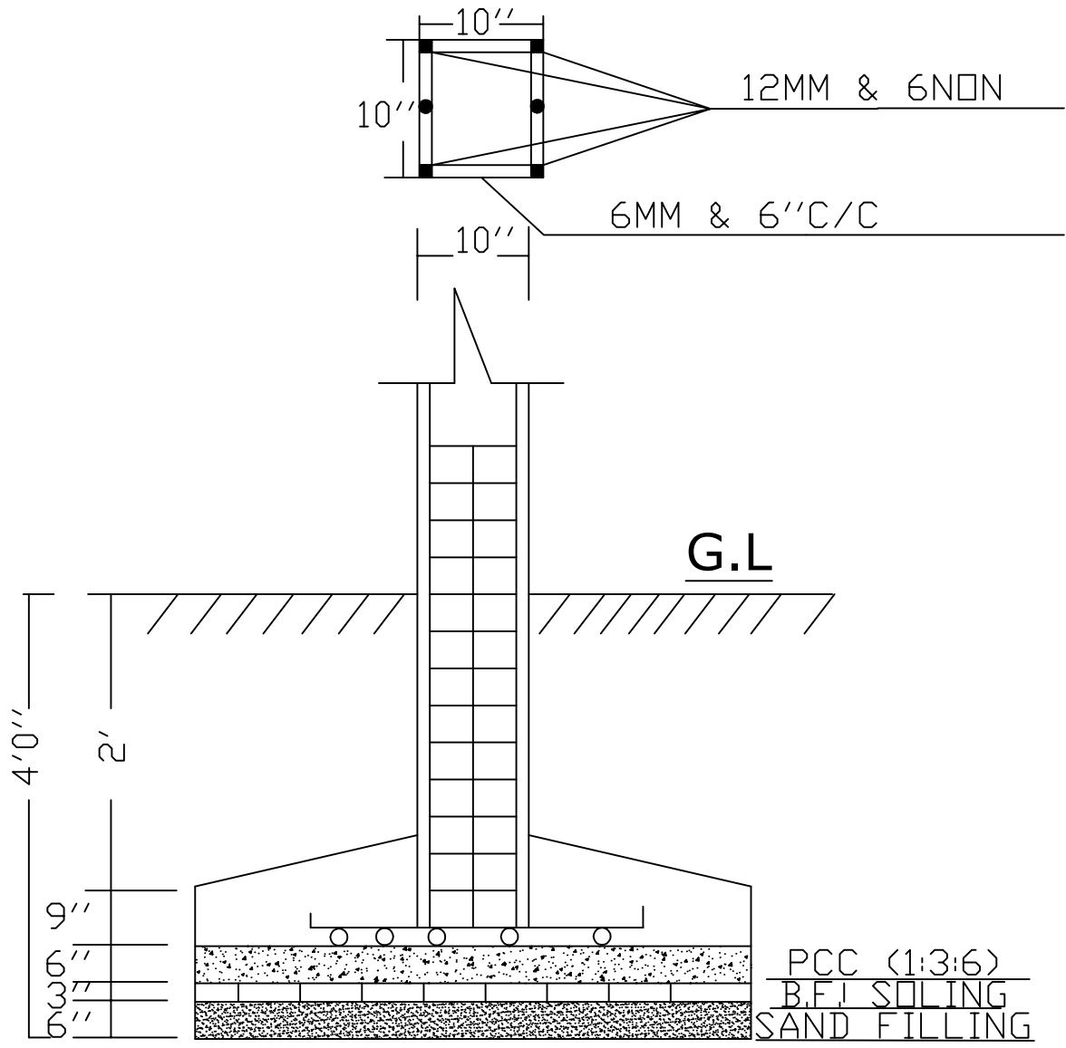
SECTION
