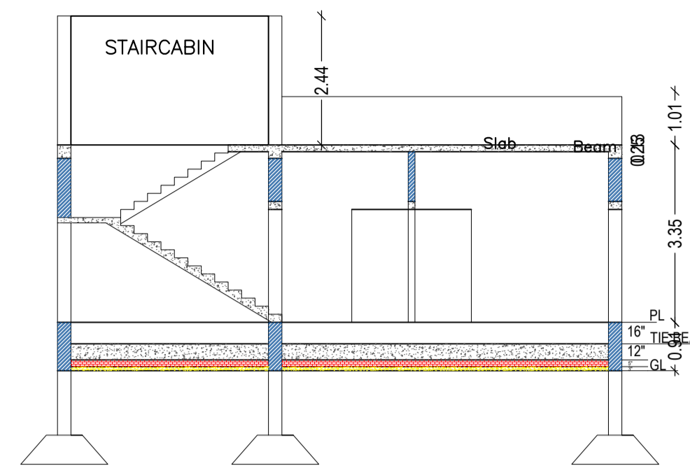
CROSS SECTION (A)
