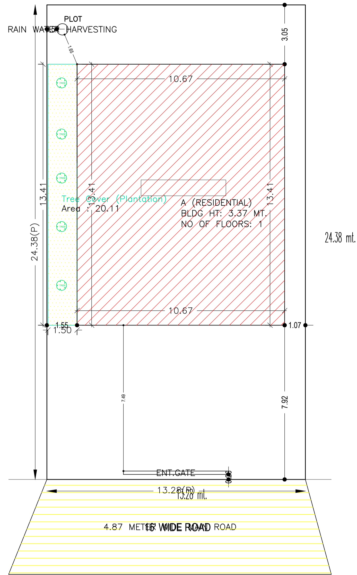
SITE PLAN
