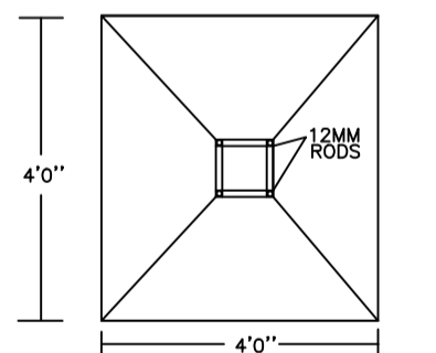
PLAN (SCALE 1"=4')
