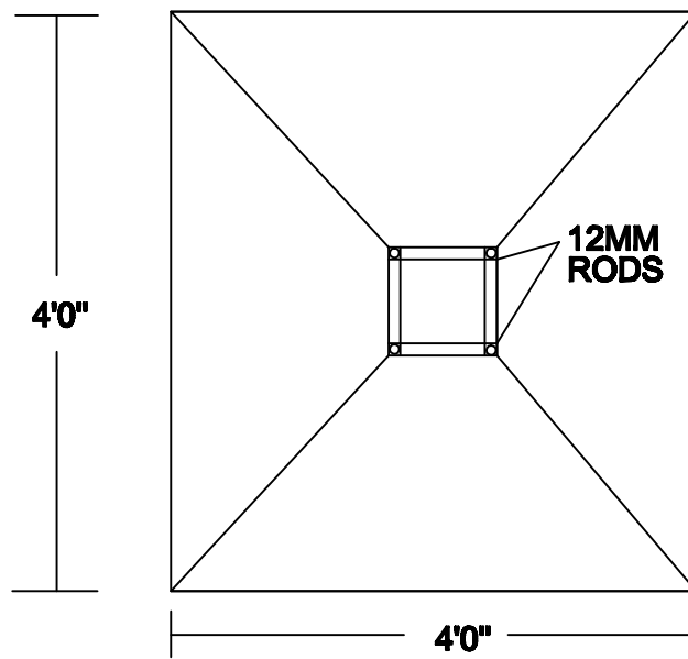
PLAN ( SCALE 1"=4' )
