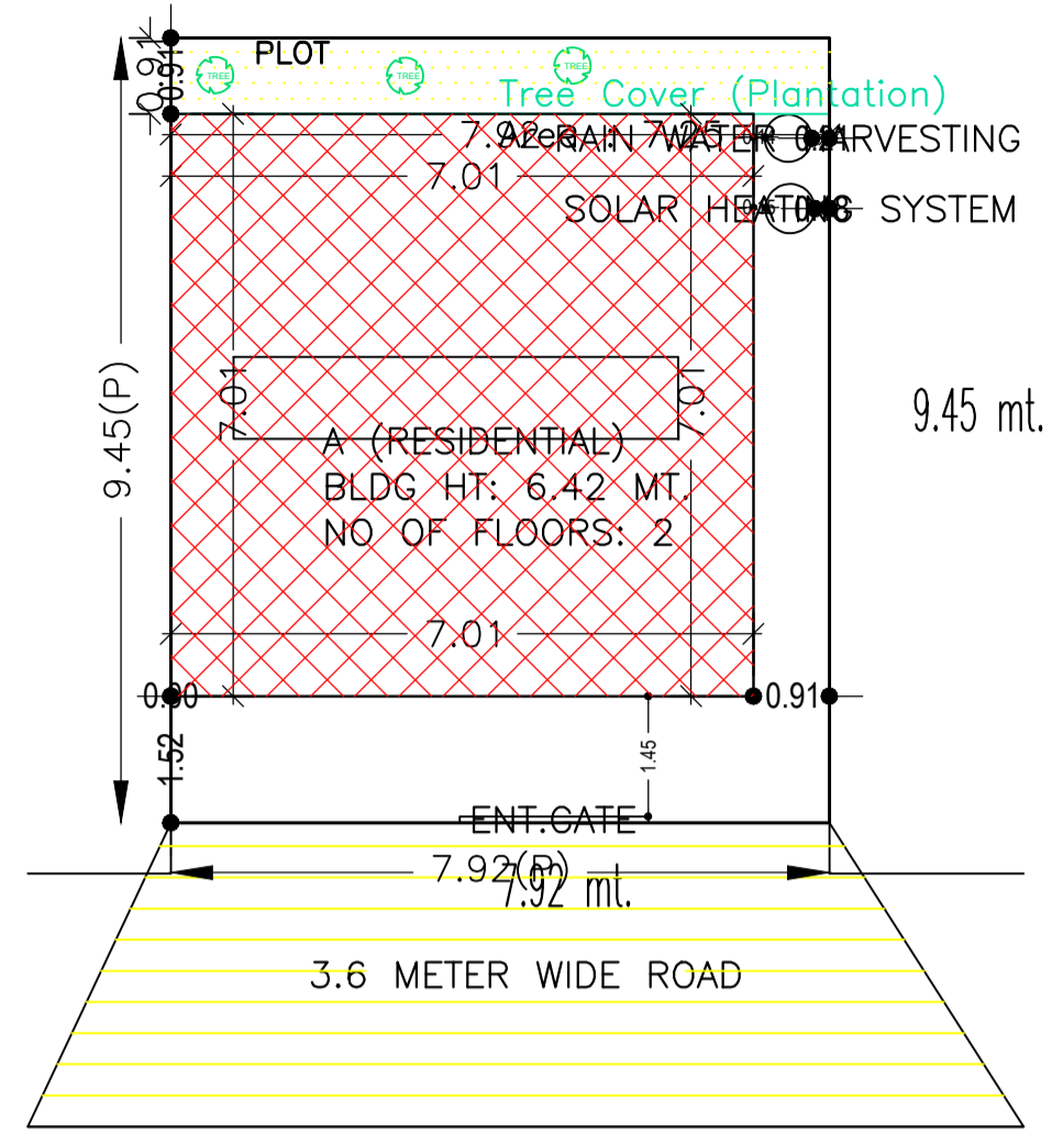
SITE PLAN
