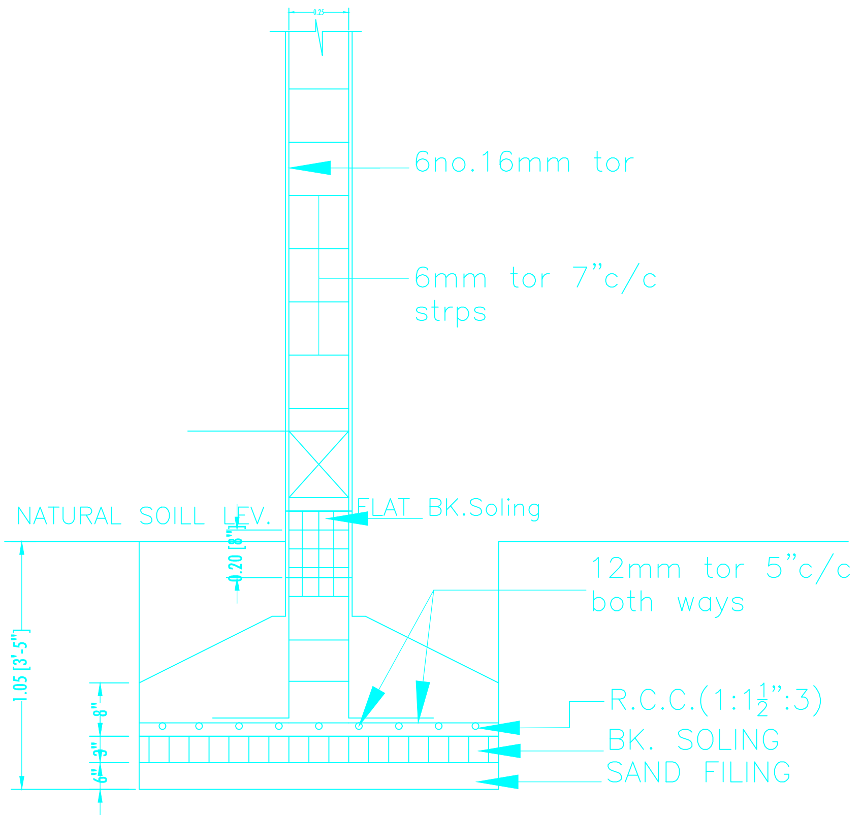
SEC. X-Y R.C.C. COLUMN FDN.DETAIL
