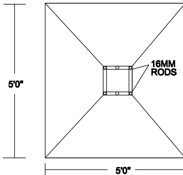
PLAN ( SCALE 1"=4' )
