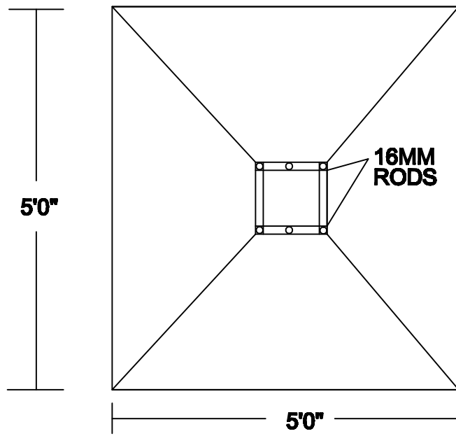
PLAN ( SCALE 1"=4' )
