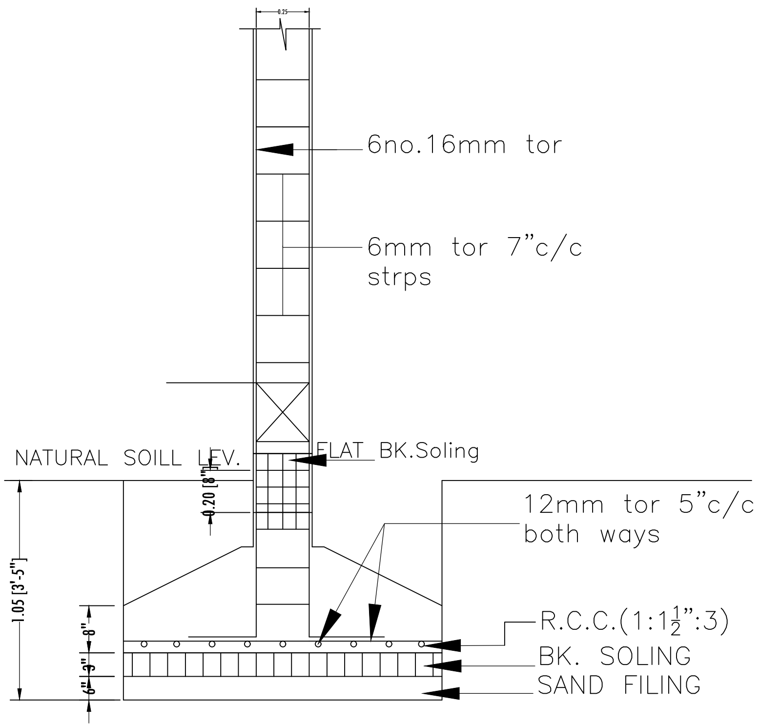
SEC. X-Y R.C.C. COLUMN FDN.DETAIL SCALE 1" = 2'-0"
