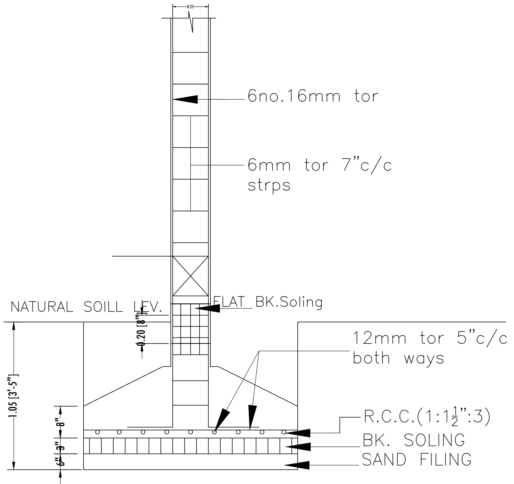
SEC. X-Y R.C.C. COLUMN FDN.DETAIL SCALE 1" = 2'-0"
