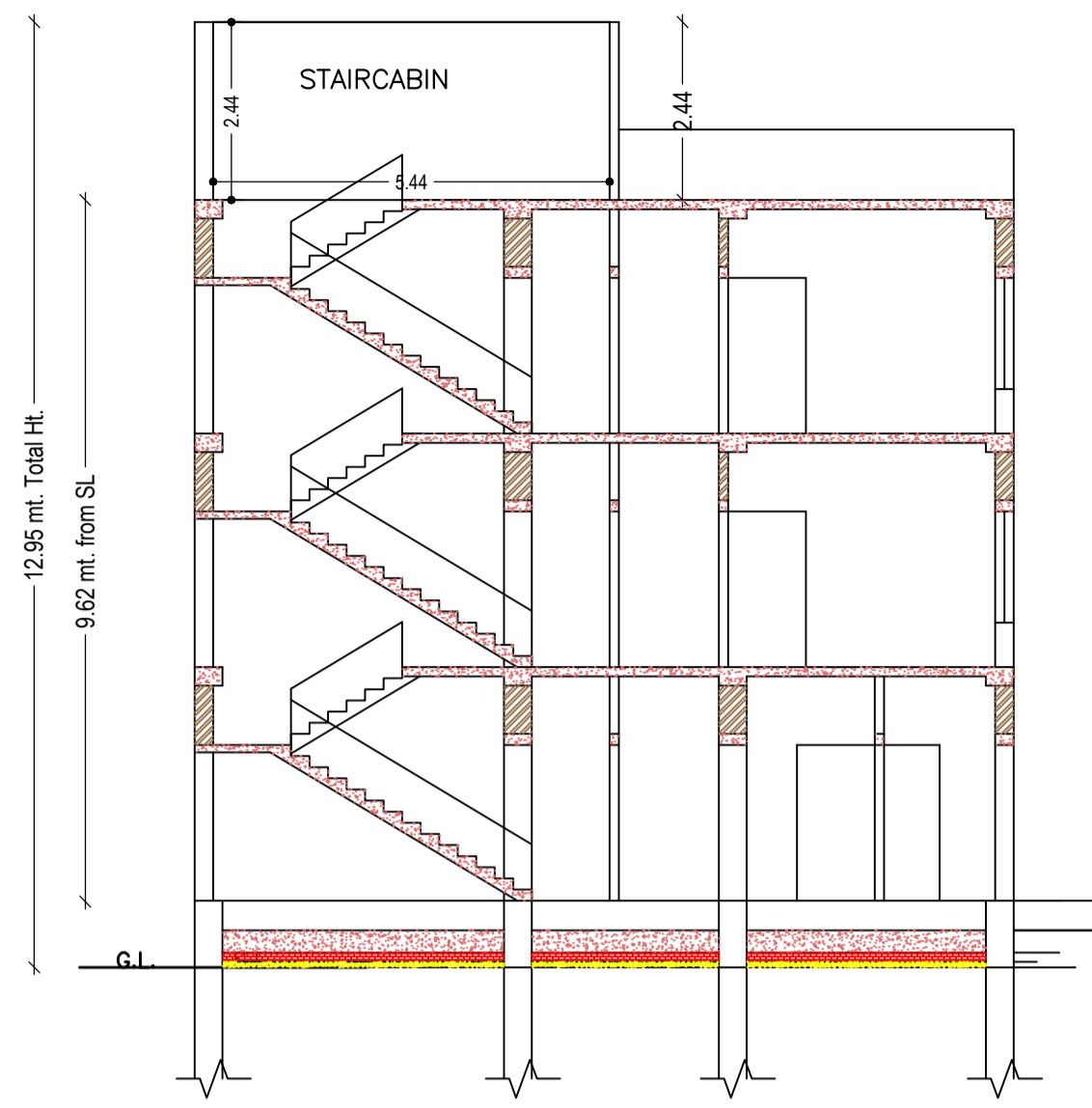
CROSS SECTION (A)
