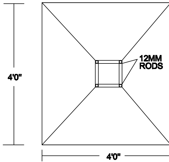
PLAN ( SCALE 1"=4' )
