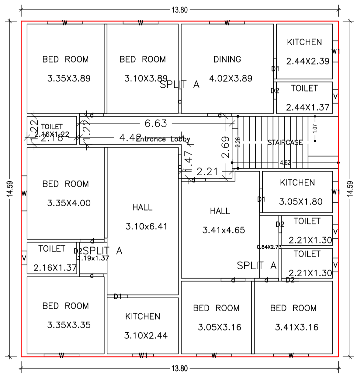
TYPICAL - 1-3 FLOOR PLAN (Proposed) (SCALE 1:100)
