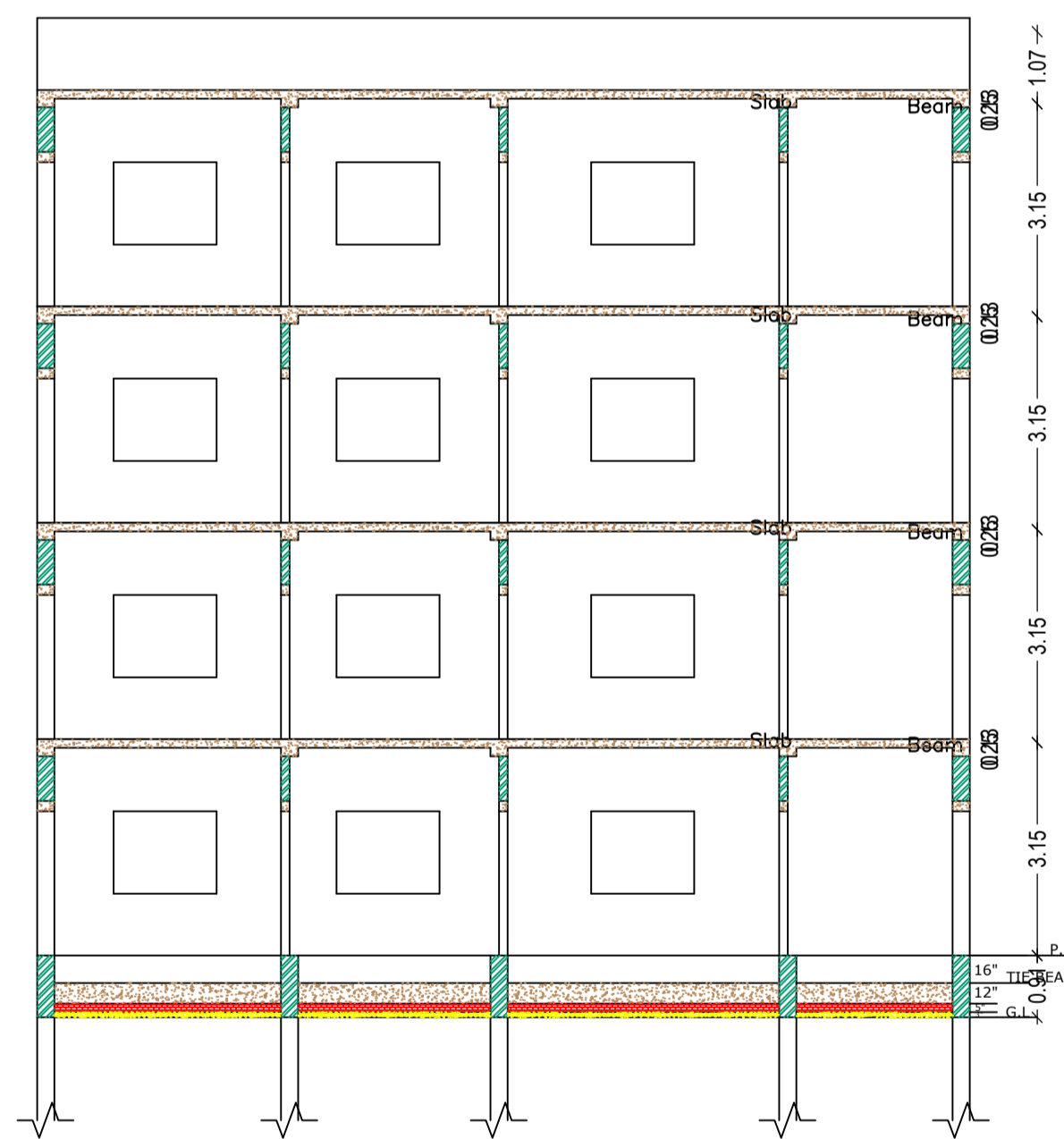
CROSS SECTION (B)
