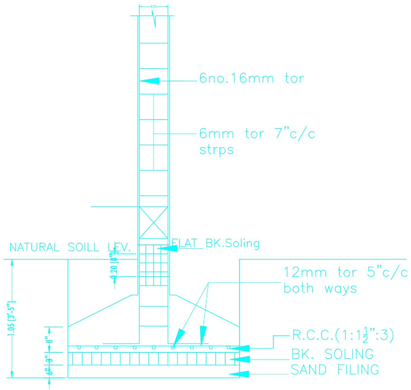
SEC. X-Y R.C.C. COLUMN FDN.DETAIL
