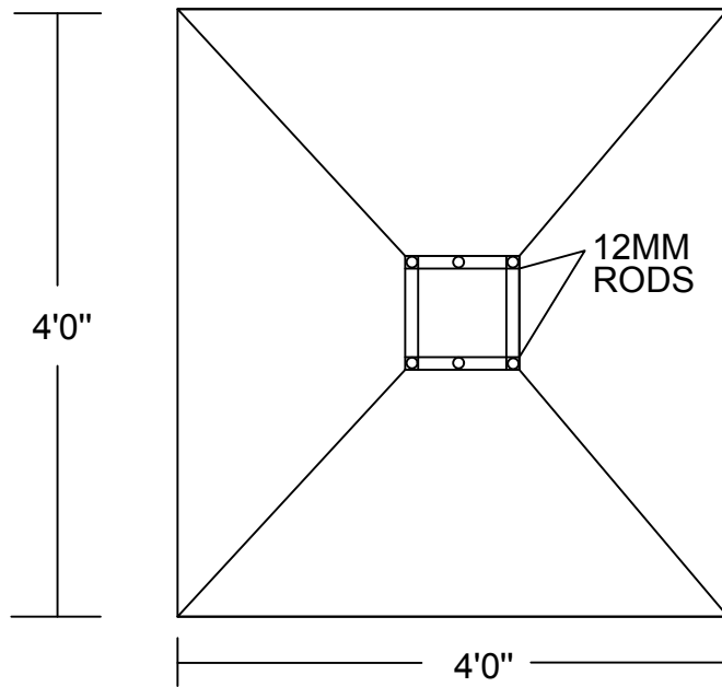
PLAN ( SCALE 1"=4' )
