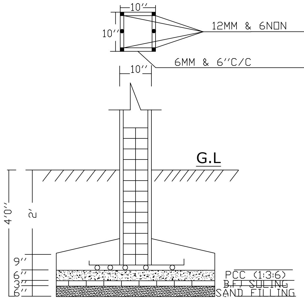
SECTION
