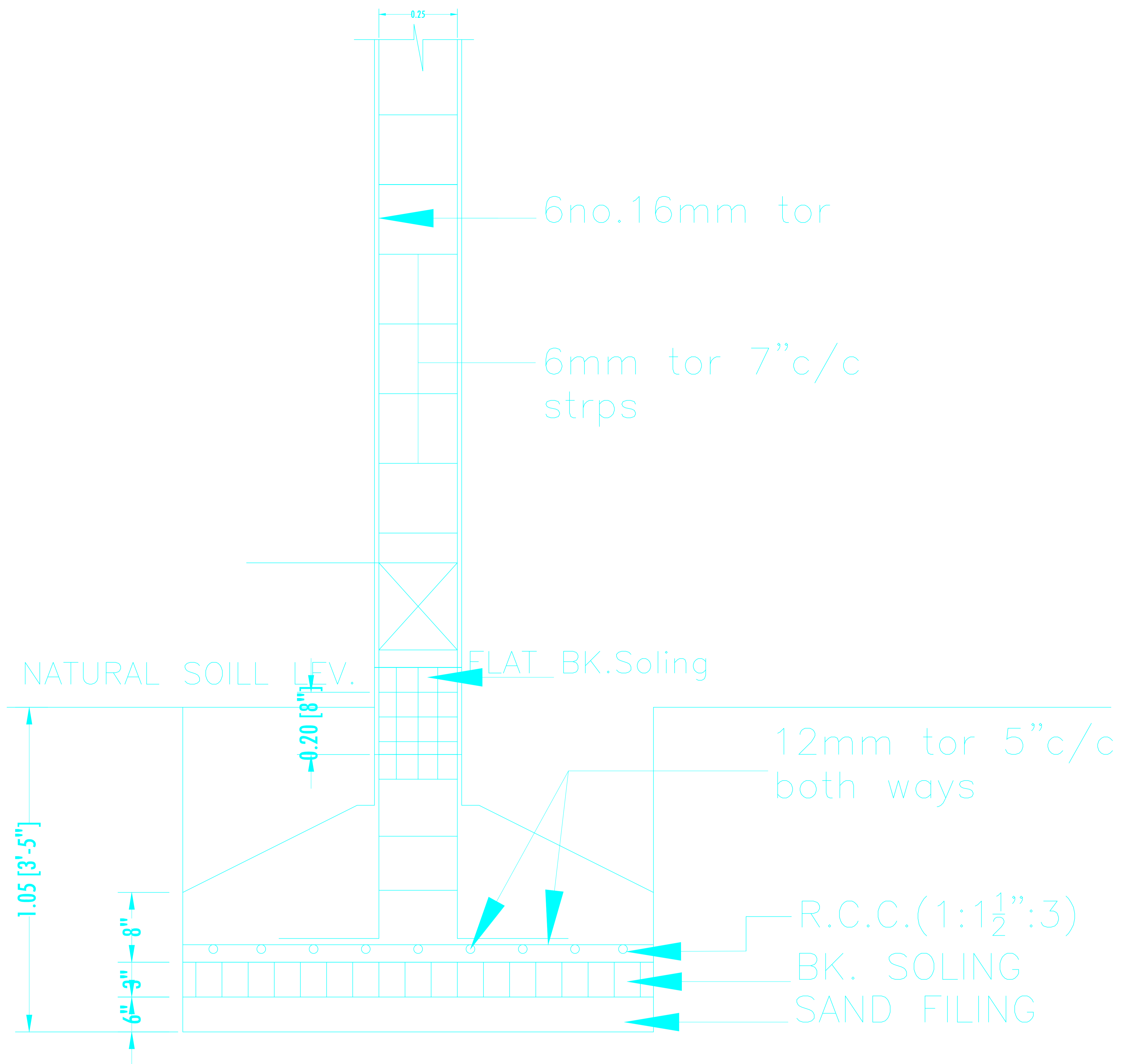
SEC. X-Y R.C.C. COLUMN FDN.DETAIL
