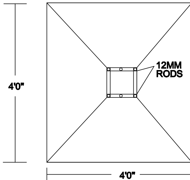
PLAN ( SCALE 1"=4' )
