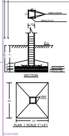
Structure Detail
