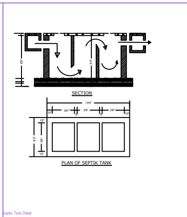
Septic Tank Detail
