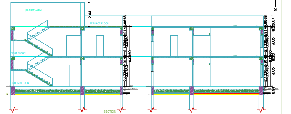
CROSS SECTION (A)
