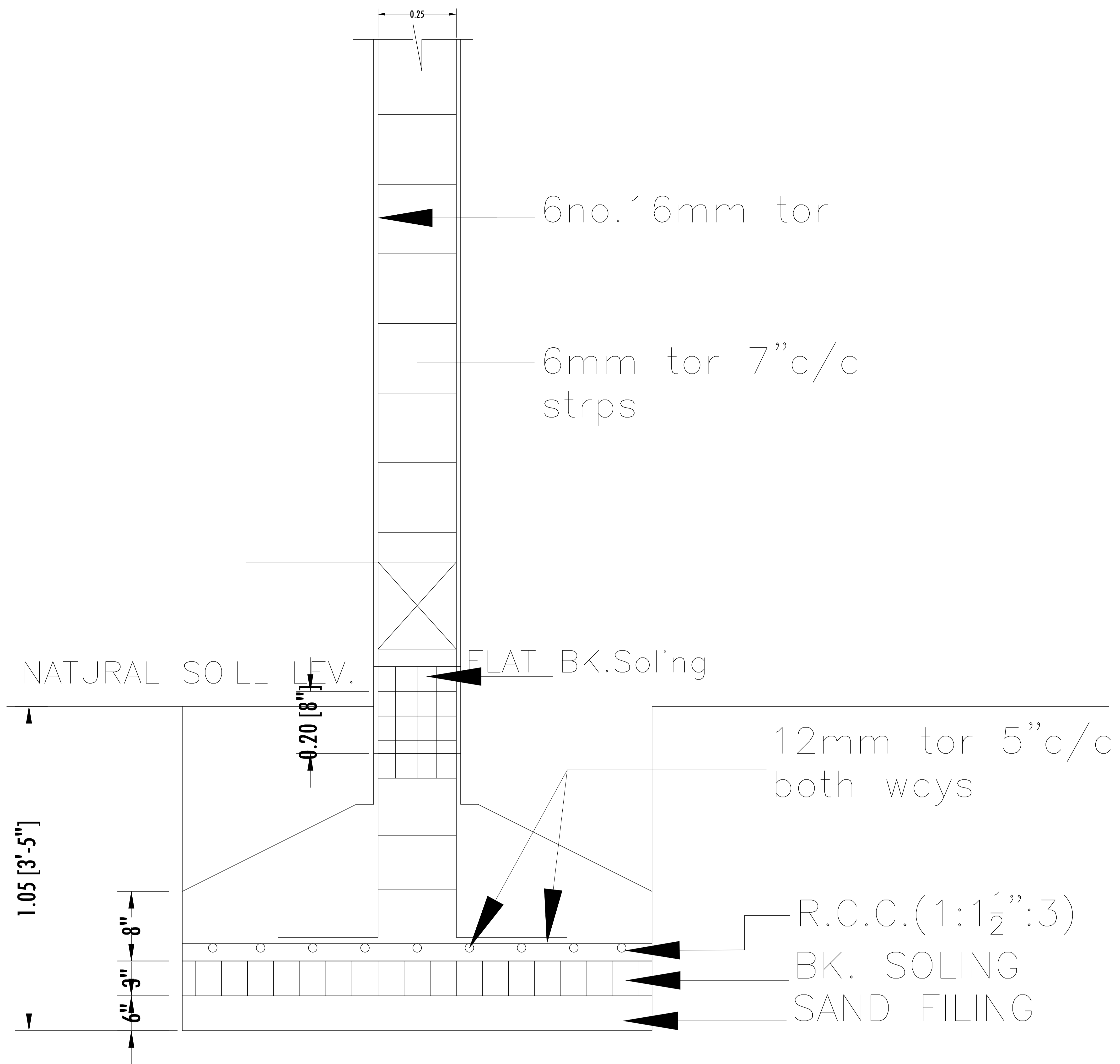
SEC. X-Y R.C.C. COLUMN FDN.DETAIL
