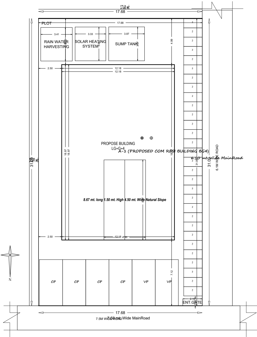
SITE PLAN
