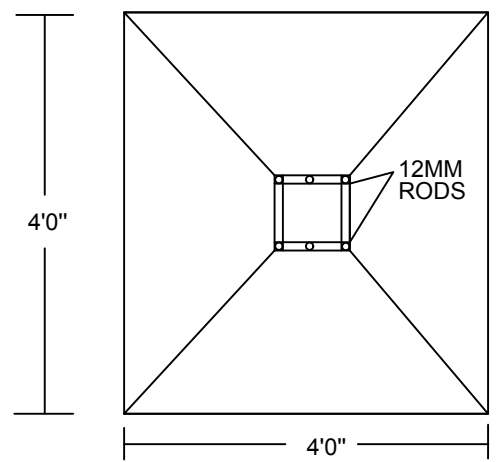
PLAN ( SCALE 1"=4' )
