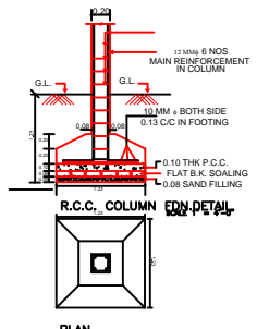
R.C.C. COLUMN WITH PETAL
