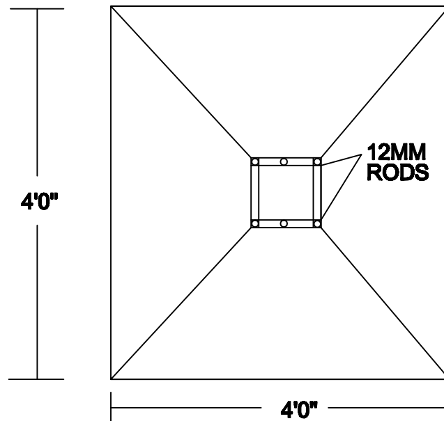
PLAN ( SCALE 1"=4' )
