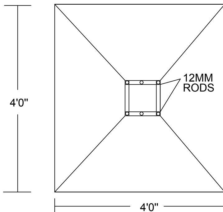
PLAN ( SCALE 1"=4' )
