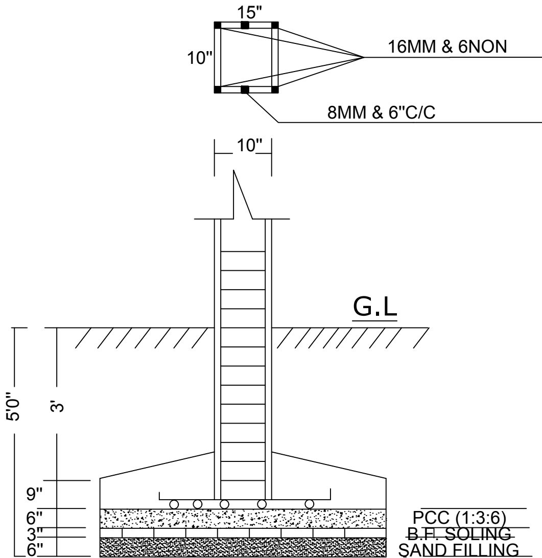
SECTION
