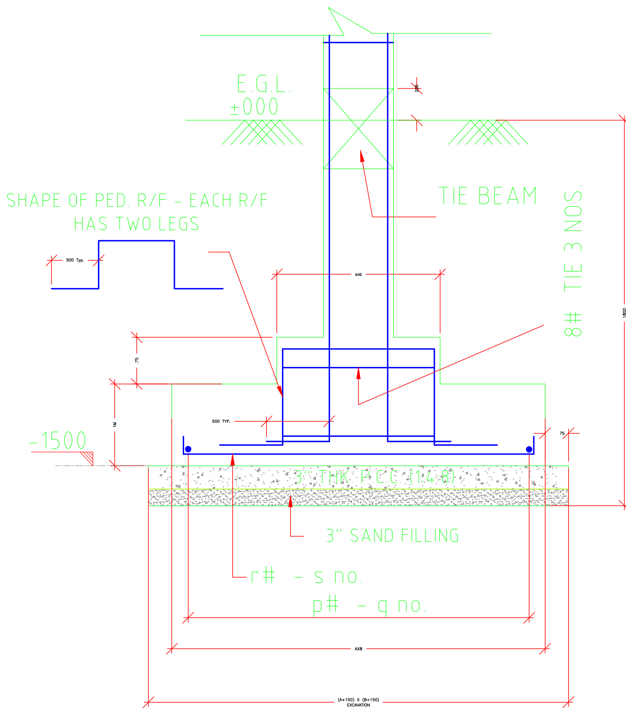
SECTION 1-1
