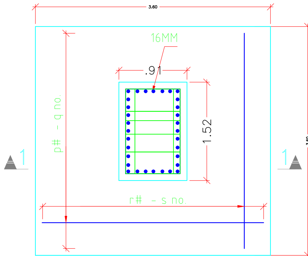
PLAN OF TYP. ISOLATED FOOTING
