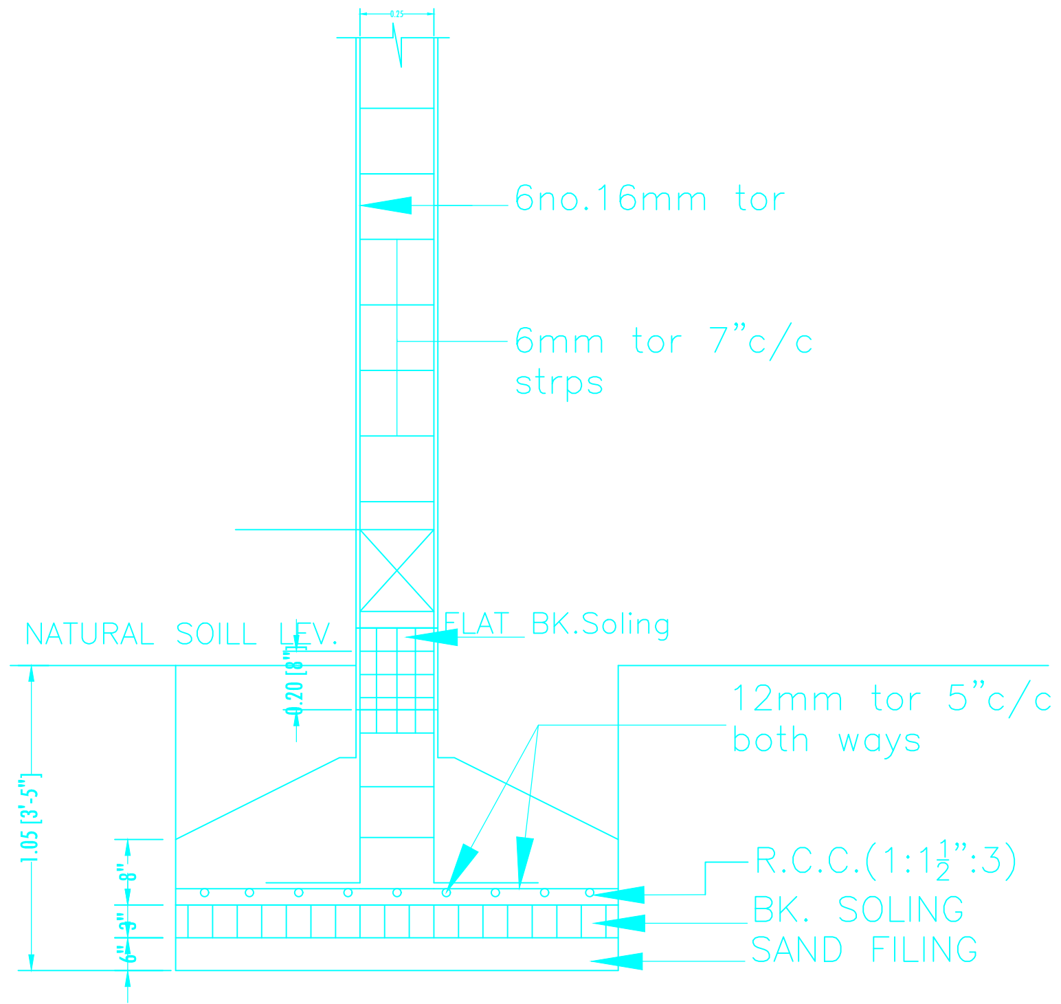
SEC. X-Y R.C.C. COLUMN FDN.DETAIL
