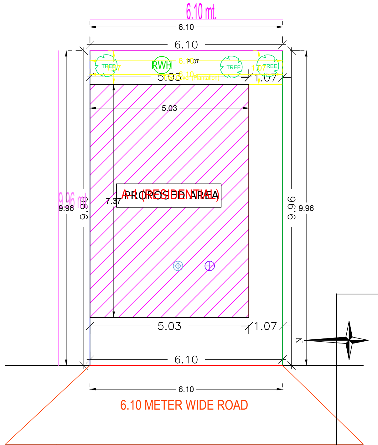
SITE PLAN
