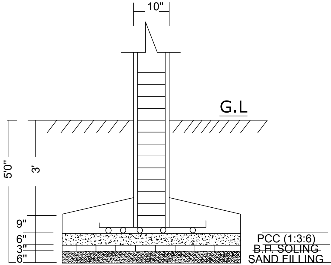
SECTION
