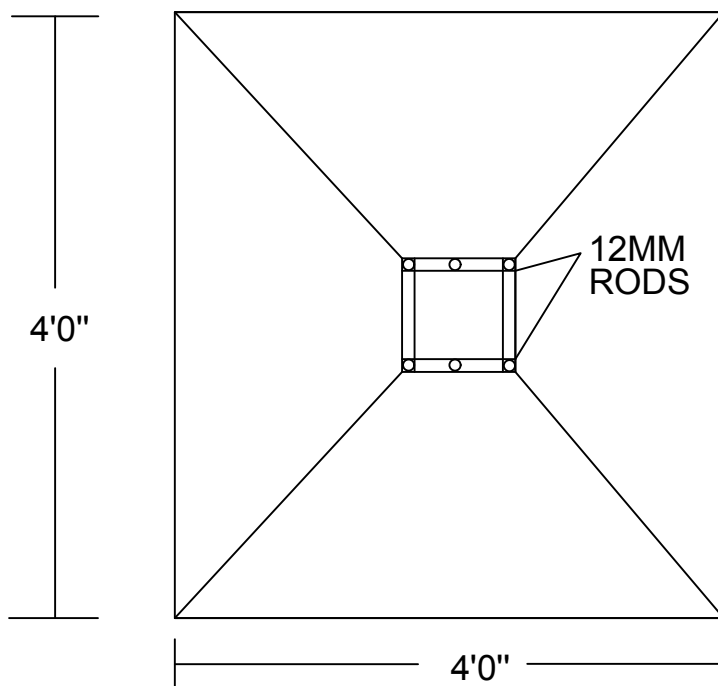
PLAN ( SCALE 1"=4' )
