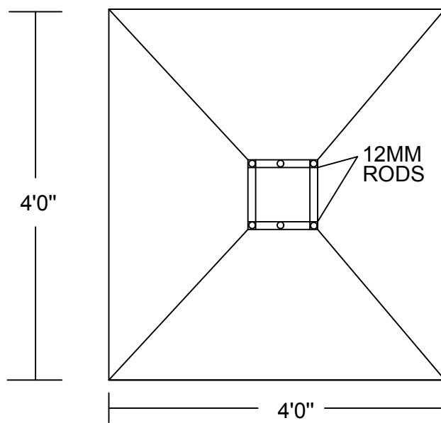
PLAN ( SCALE 1"=4' )
