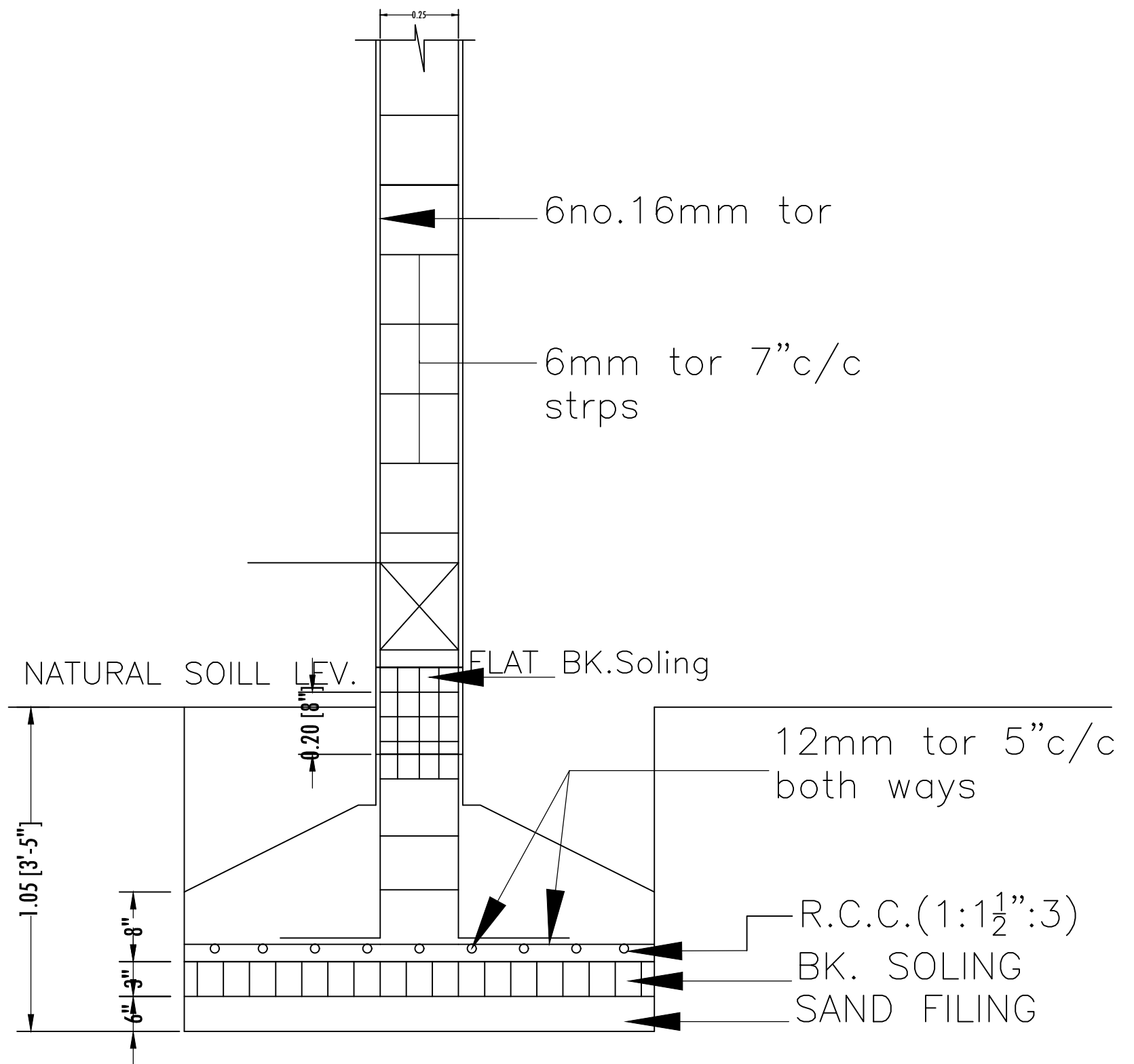
SEC. X-Y R.C.C. COLUMN FDN.DETAIL
