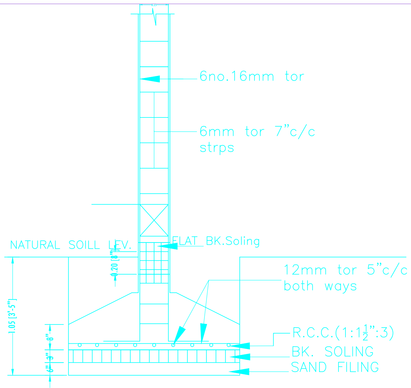
SEC. X-Y R.C.C. COLUMN FDN.DETAIL SCALE 1" = 2'-0"
