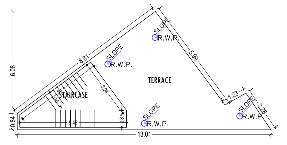
THIRD FLOOR PLAN (Proposed) (SCALE 1:100)
