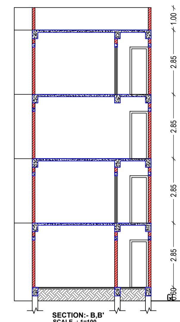
SECTION - B-B' SCALE - 1:100
