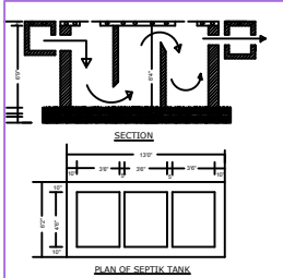
Septic Tank Detail
