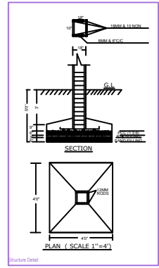
Structure Detail
