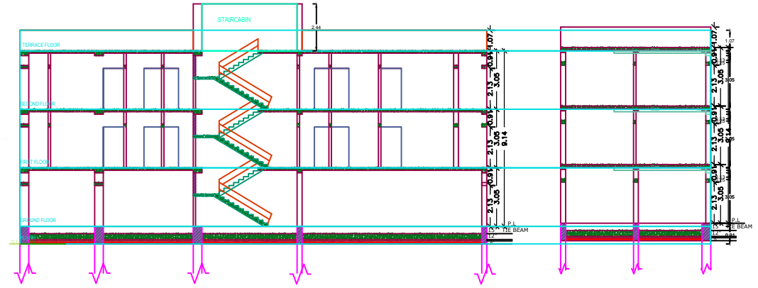
CROSS SECTION (A)
