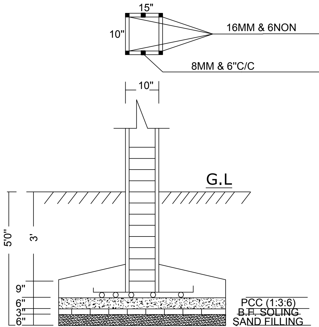
SECTION
