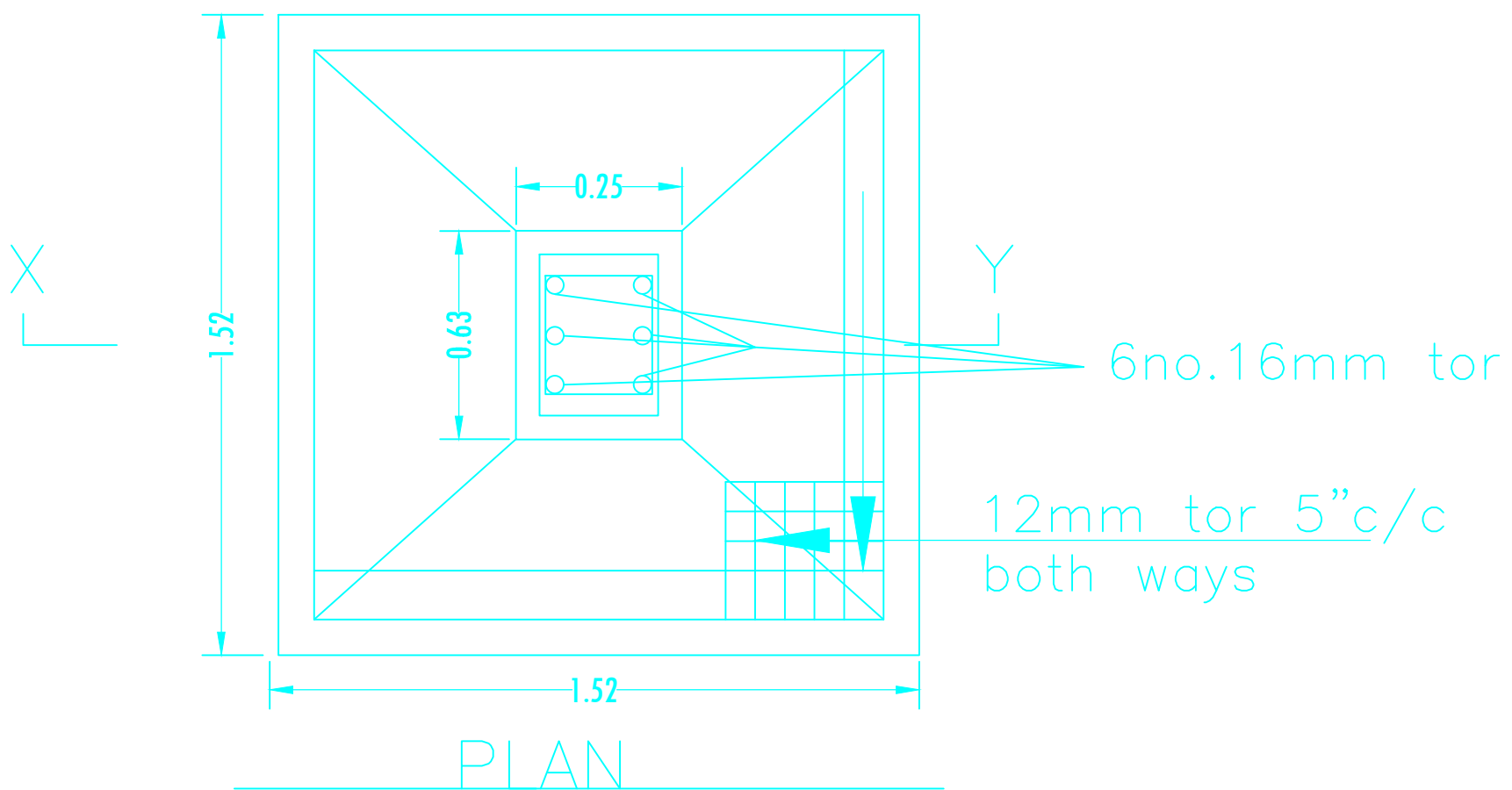
SCALE-1":2'-0"
