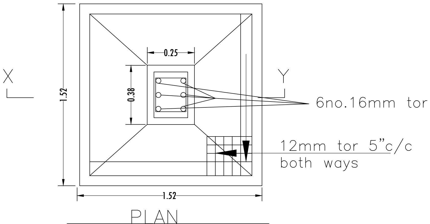
SCALE - 1":2'-0"
