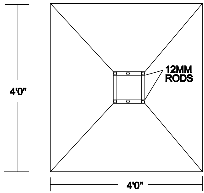
PLAN ( SCALE 1"=4' )
