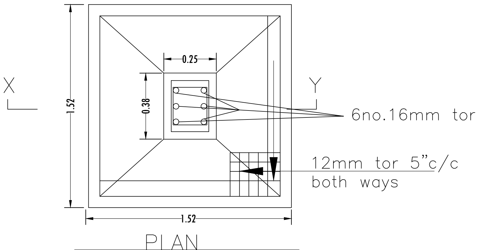
SCALE-1":2'-0"
