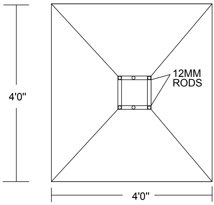
PLAN ( SCALE 1"=4' )
