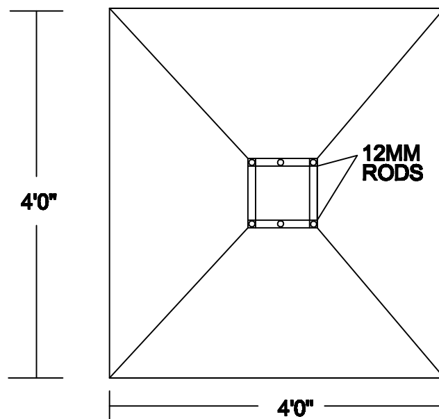
PLAN ( SCALE 1"=4' )
