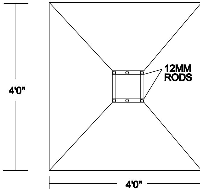
PLAN ( SCALE 1"=4' )
