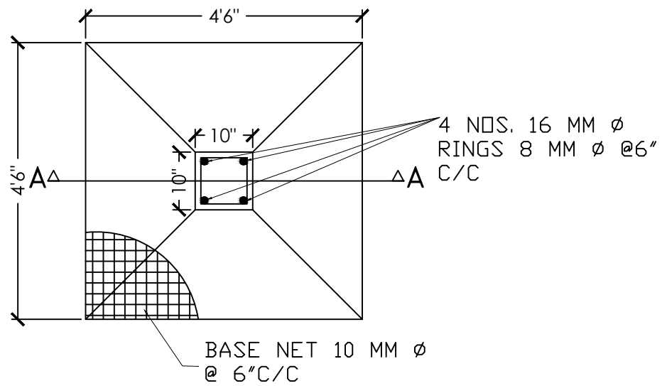
PLAN OF COLUMN FOUNDATION
