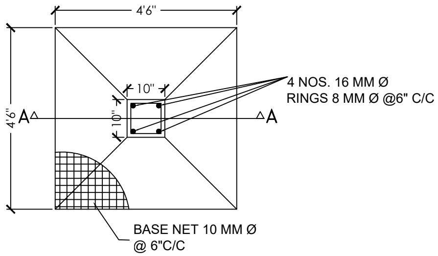
PLAN OF COLUMN FOUNDATION
