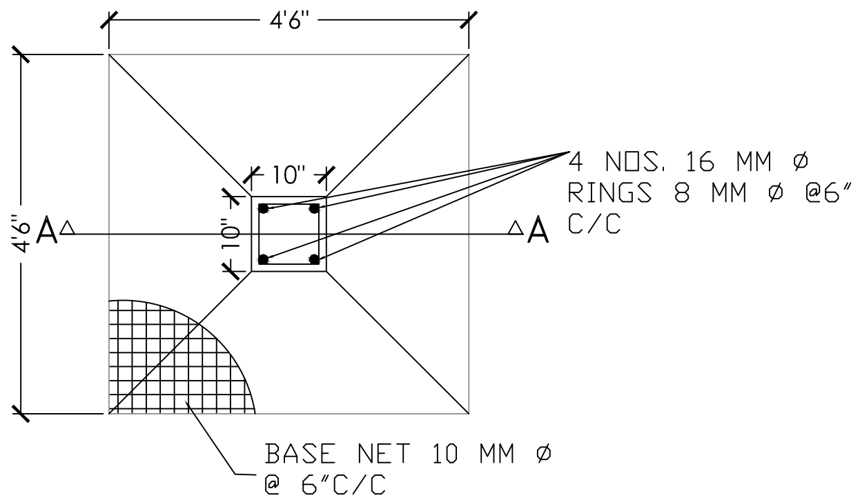
PLAN OF COLUMN FOUNDATION
