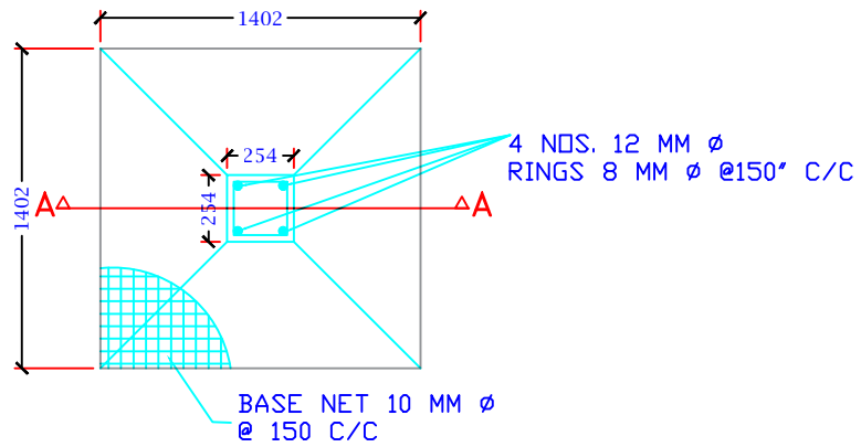
PLAN OF COLUMN FOUNDATION
