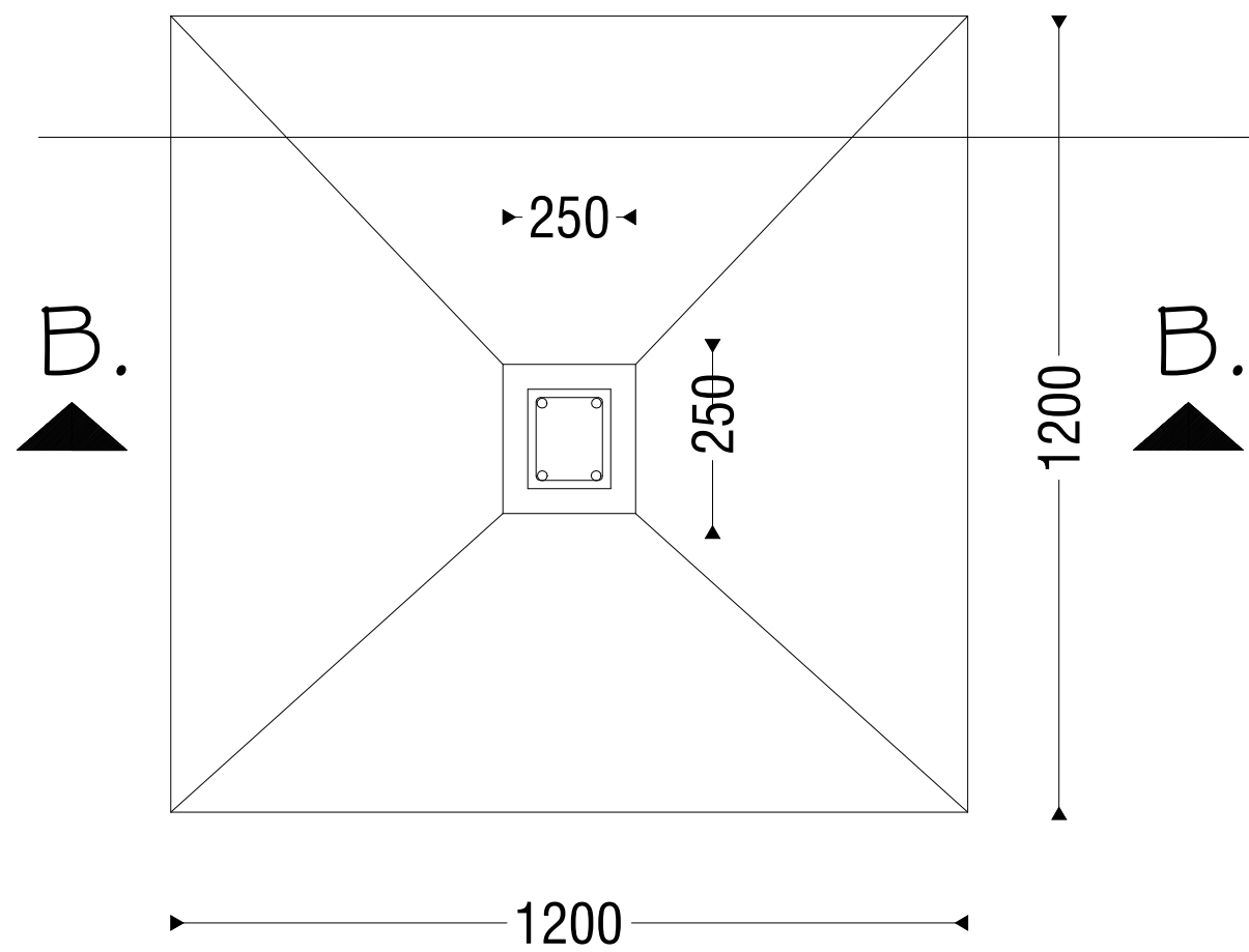
DETAIL OF FOUNDATION
