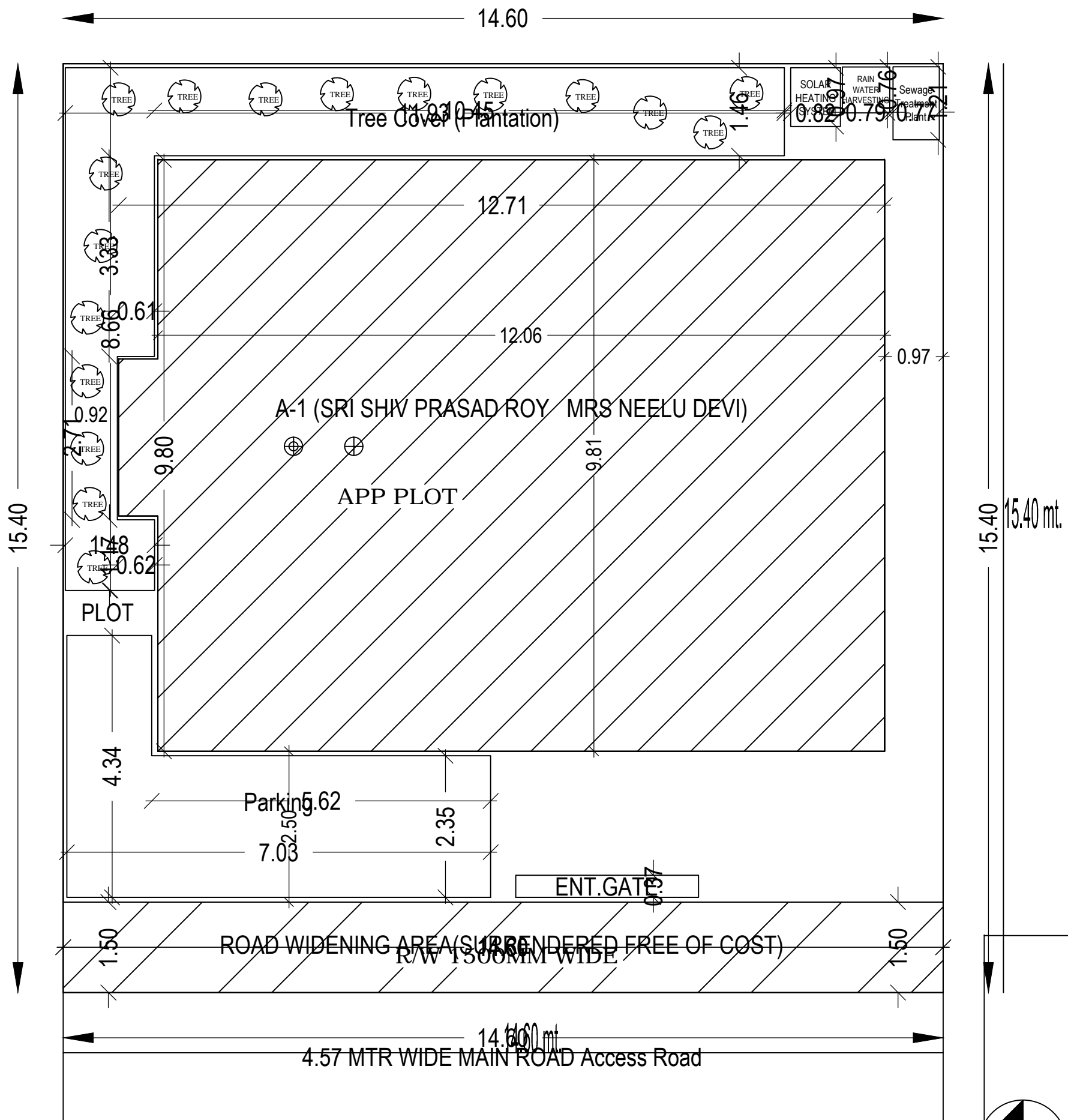
SITE PLAN
