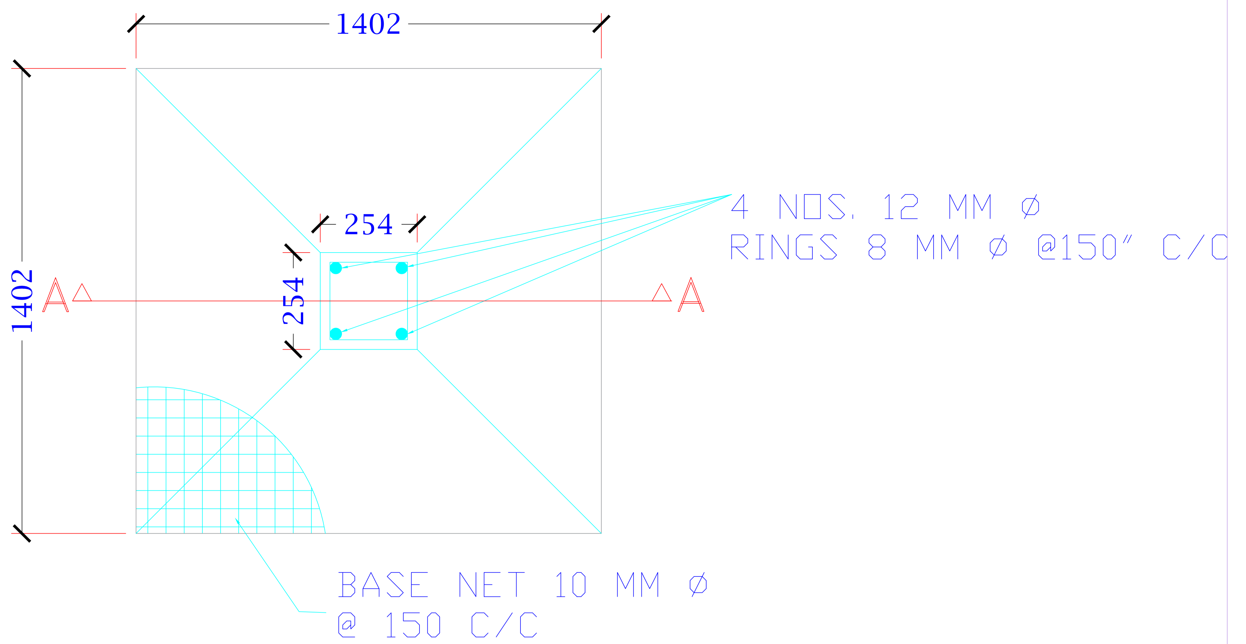
PLAN OF COLUMN FOUNDATION
